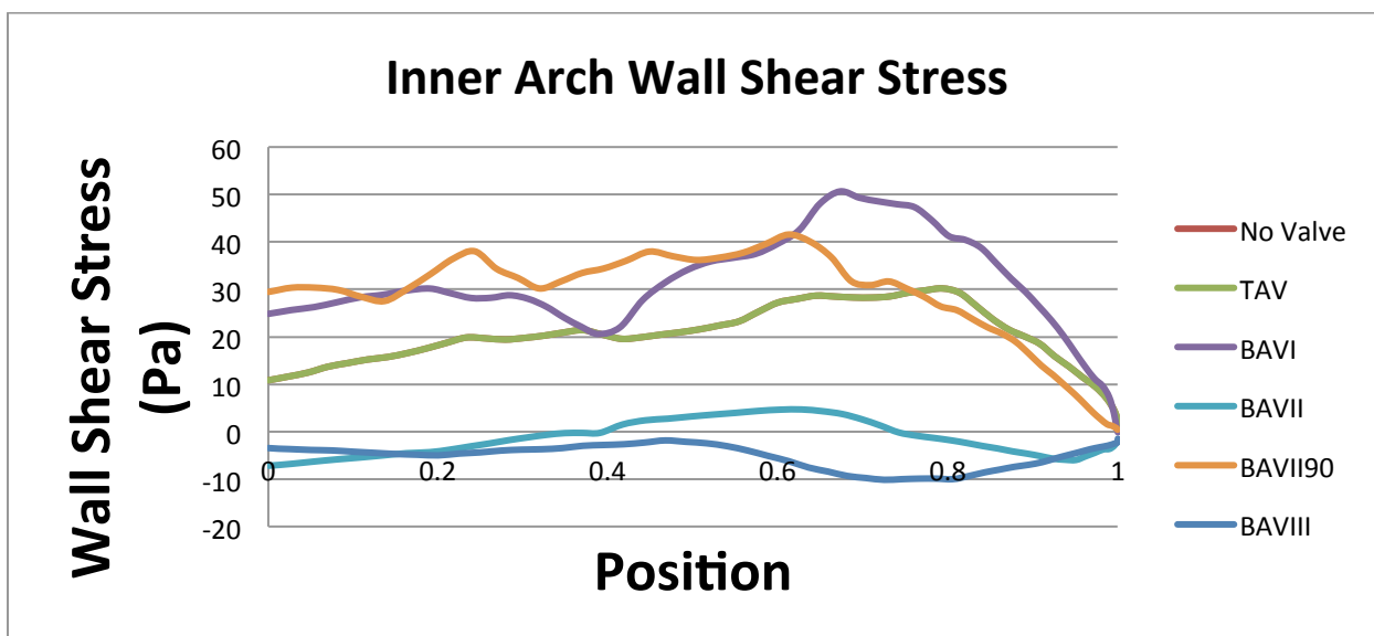
Figure 17. Position along inner arch in axial direction versus WSS magnitude
